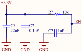
Boot Delay Circuit
