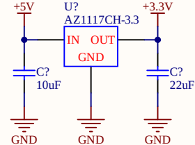
USB Power Regulator
