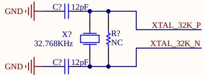
RTC Crystal
