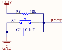
Boot Switch
