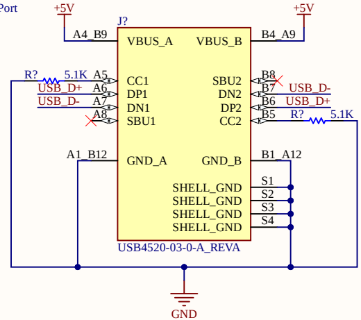
USB Port
