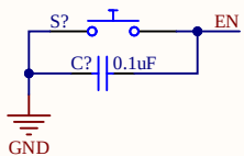
Reset Switch
